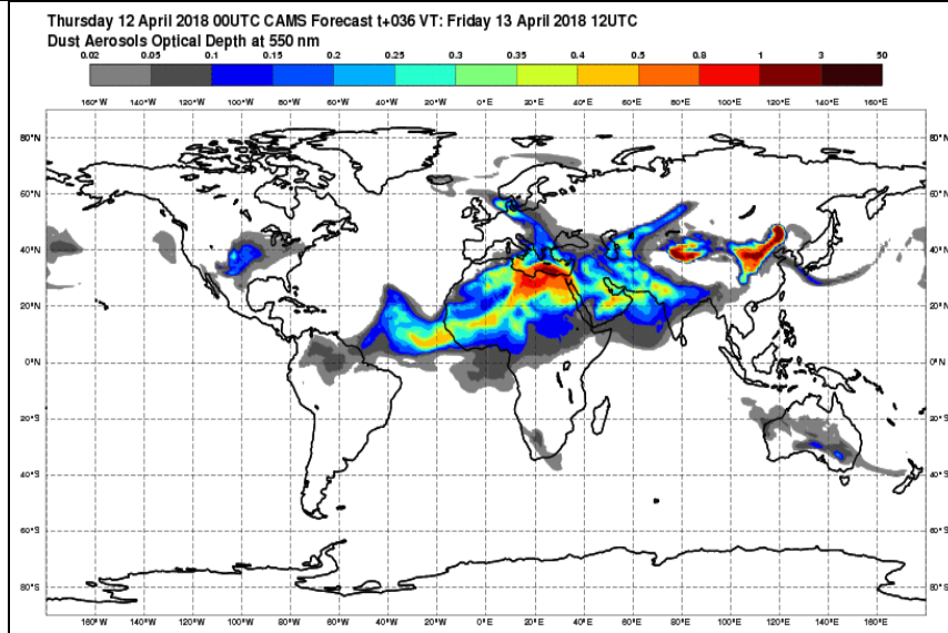
Dust Forecast
