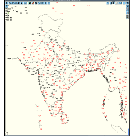
Tendency MSLP
