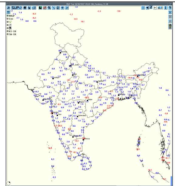
Tendency MSLP
