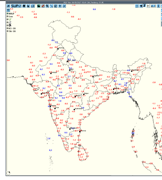
Tendency MSLP
