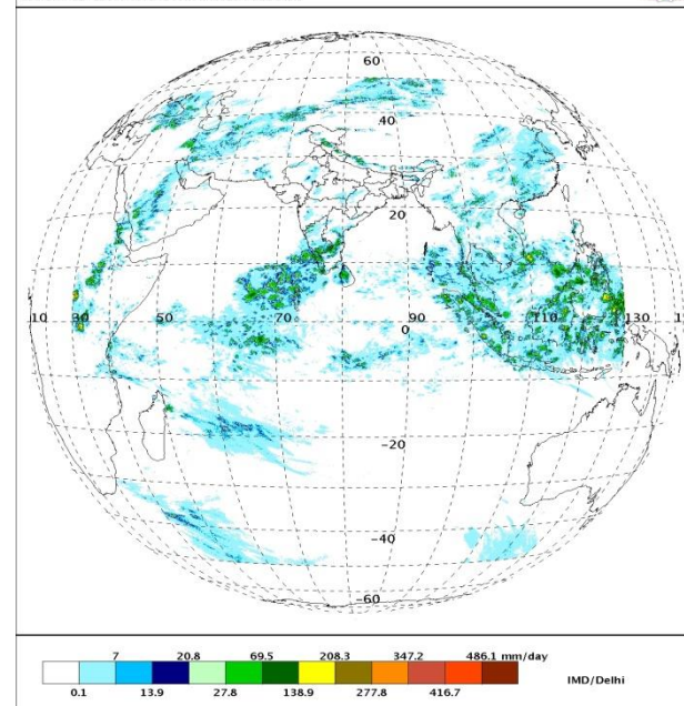
HEM Rainfall
