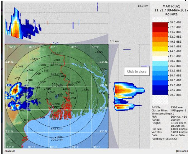
DWR Kolkata at 1121 UTC (1651hrs IST) of today
