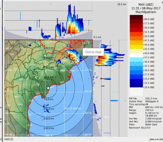
DWR Machilipatnam at 1131 UTC (1701 hrs IST) of today
