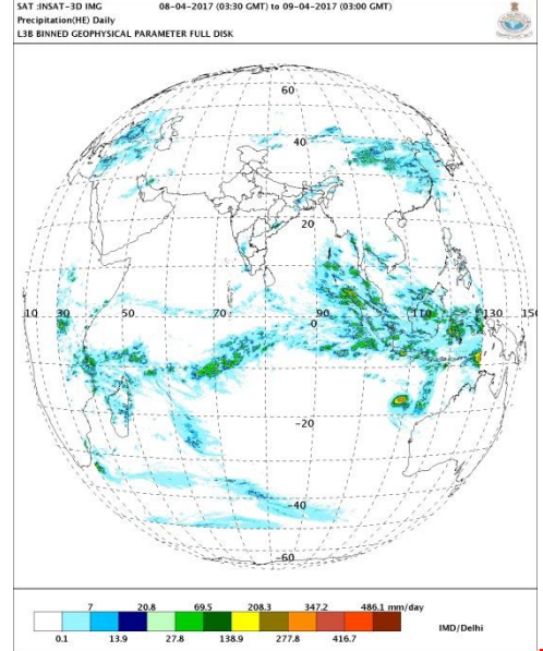
HEM Rainfall
