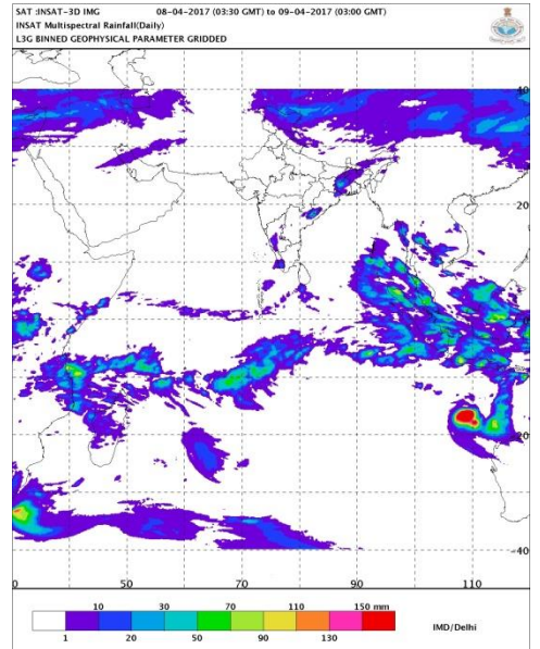
IMR Rainfall
