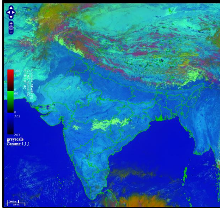
RAPID RGB Imagery at 1030IST of the Day
