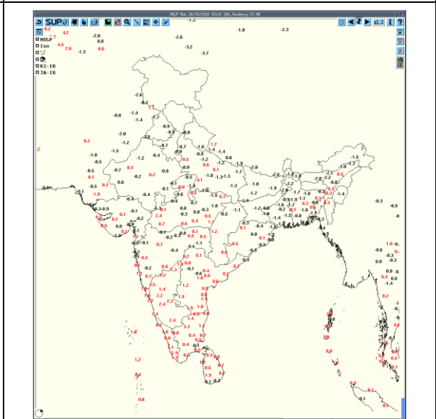
Tendency MSLP
