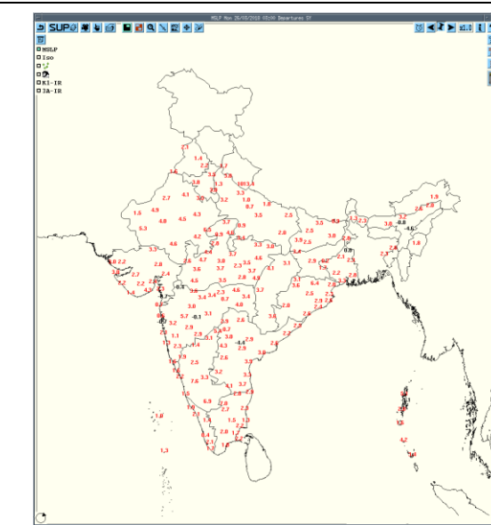
Departure MSLP
