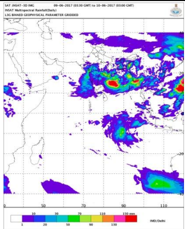
IMR Rainfall
