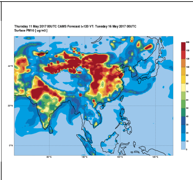
PM10 Forecast for 00UTC of 16 th May
