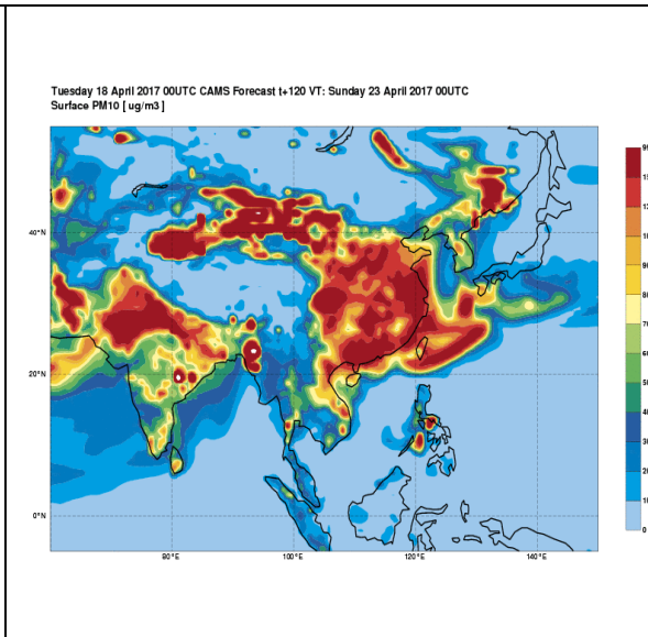
PM10 Forecast for 00UTC of 23rd April
