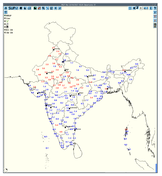
Departure MSLP
